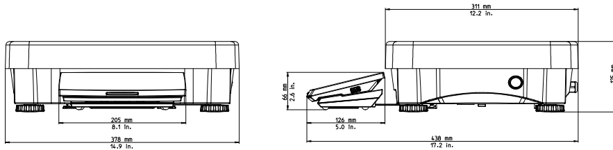
Figure 9-3. EXP24001, EXP35001 and EXP65001 models
