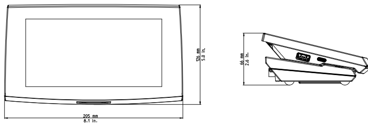
Figure 9-4. EXP Terminal
