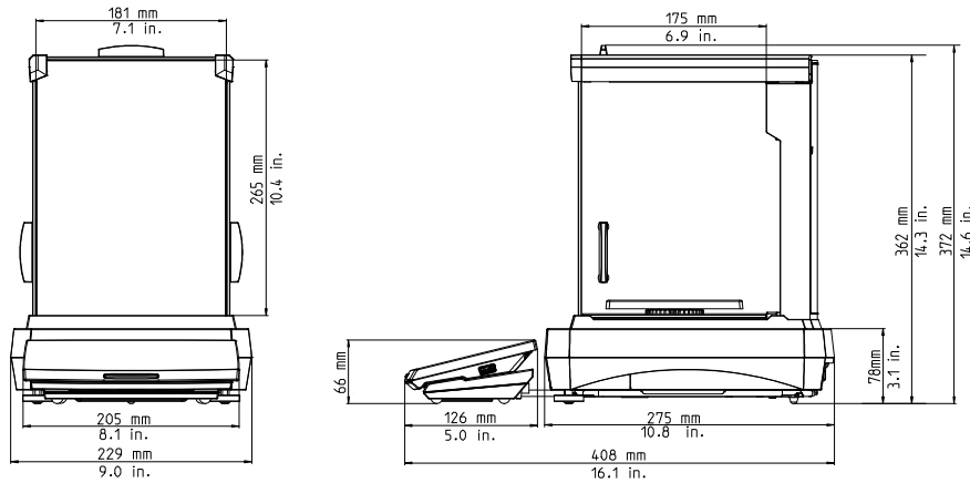
Figure 9-1. Draftshield models
