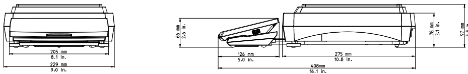
Figure 9-2. Non-Draftshield models
